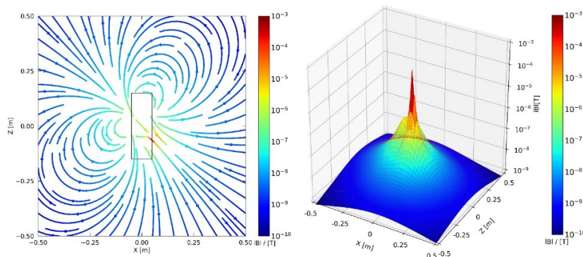
Fig. 4. Predicted magnetic field for zero field space in xz plane calculated by torque rod in the residual magnetization ( y = 0 ). The left plot is stream plot, the right plot is 3D contour plot.
